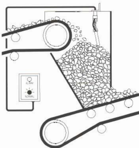
► Stortkoker of tussenbunker over-flow bewaking
